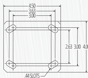
STANDARD TOP PLATE
