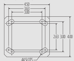
STANDARD TOP PLATE
